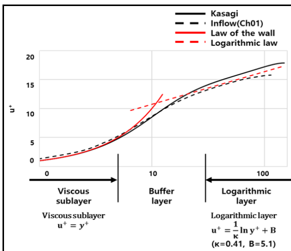
Fig 3: Comparison of u^+ Among DNS (Kasagi) Data, Synthetic Inflow Data, and Theoretical Results
