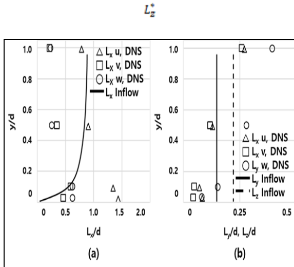
Fig 2: Profiles of integral length scales in the inlet ,
