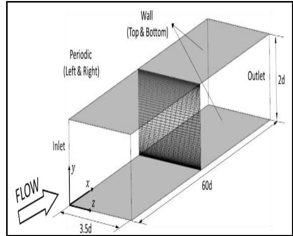
Fig 1: Schematics of computational channel domain
